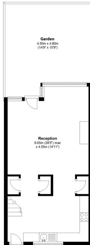
Ground Floor
